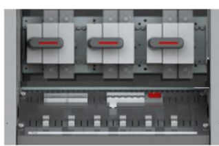
Type E Battery Switch fuses in Battery connection panel
