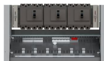
Type C Battery MCCBs in Battery connection panel
