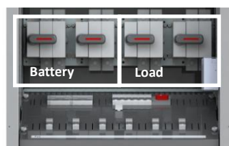
Type D Battery Switch fuses and Load Switch fuses in combined battery/load connection panel
