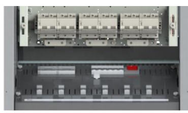
Type B Battery MCBs in Battery connection panel
